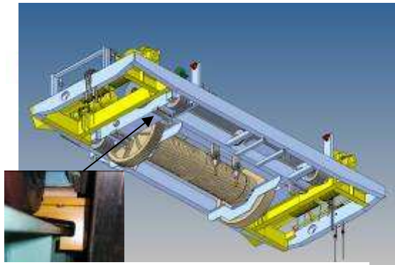
Trolley anti-derailment
