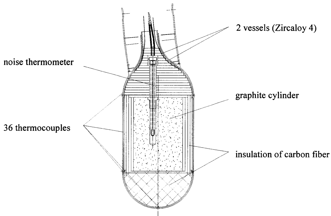
Figure 1: Hot neutron source vessels with graphite cylinder and insulation
