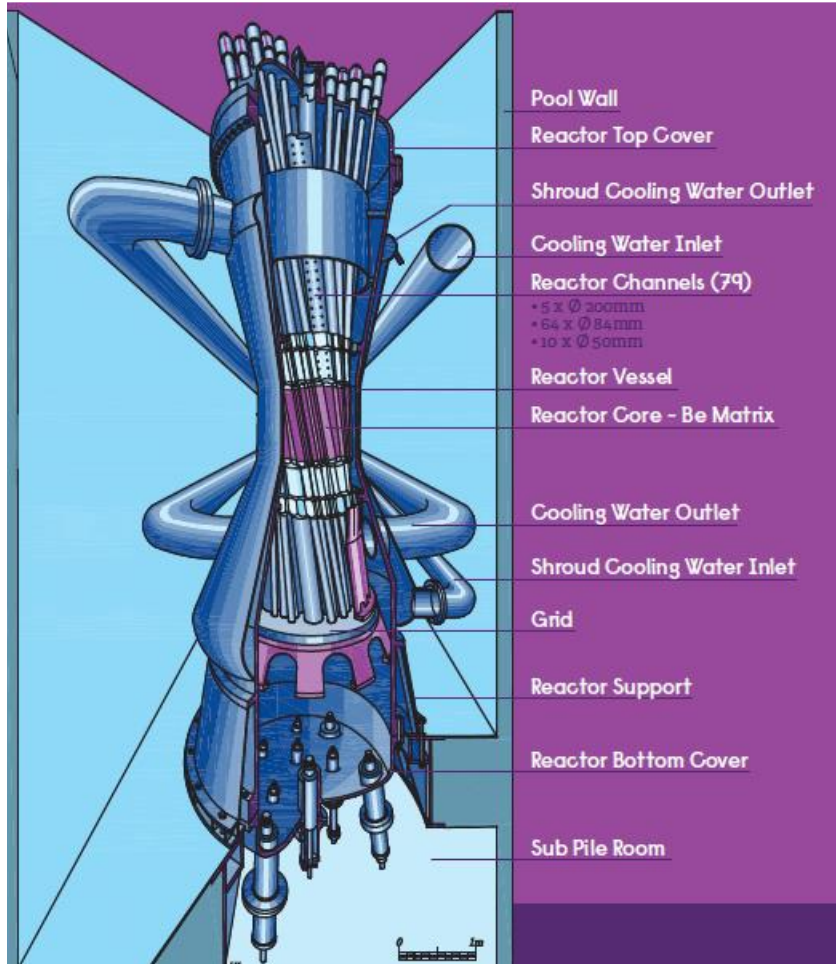
Figure 1: Lay out of the BR2 reactor, with visualisation of the 79 irradiation channels, the primary piping and the shroud cooling.
