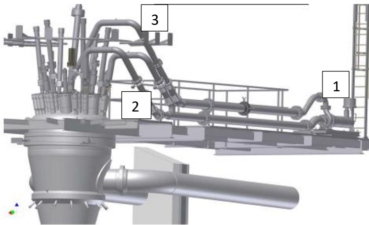
Figure 3: the EVITA loop installed in the BR2 reactor with the pump (1), the 2 feed lines and the discharge line (3) connected to the central reactor channel, containing the test section.
