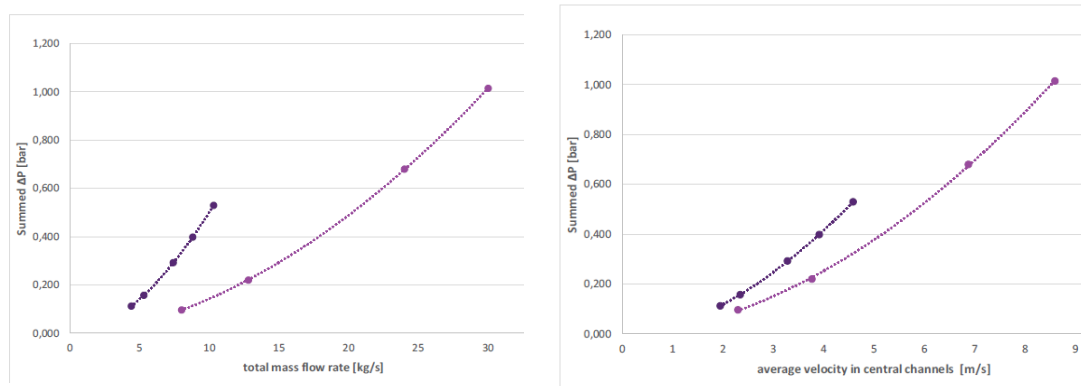
Figure 5: the calculated flow rate and velocity in 2 typical fuel assemblies in the MUSTANG-R device.
