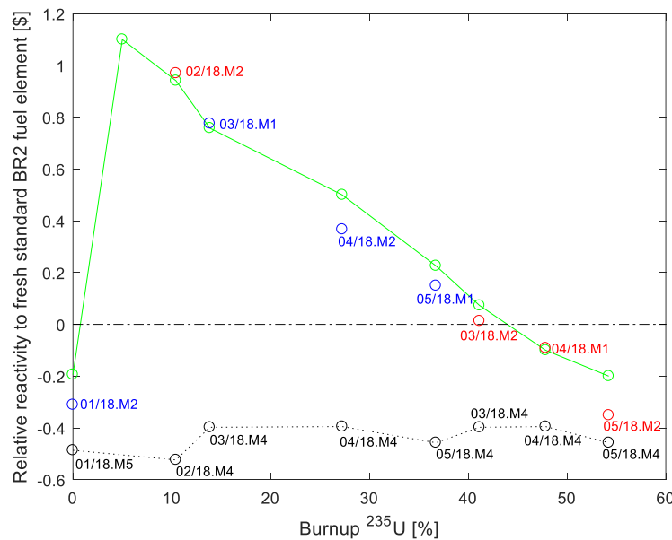
Figure 4: the calculated and measured effect of burn-up on the reactivity effect of an HEU BR2 fuel element with B and Sm as burnable absorbers versus Gd.
