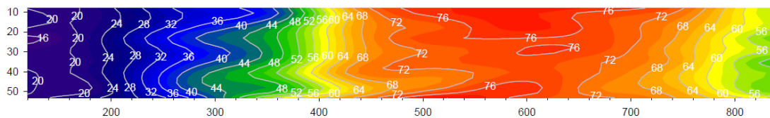
Figure 5: the calculated burn-up distribution in a high density silicide fuel plate, irradiated in the FUTURE basket for 88 days.
