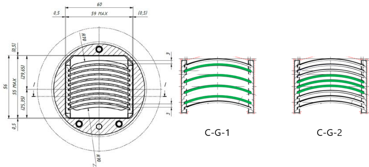
Figure 2: design of the generic test assembly cross section (left); the variants to the right allow for larger coolant flow gaps and less plates in the fueled plates.
