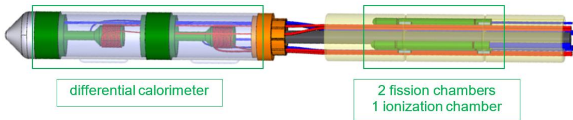
Figure 4: Measuring cell
