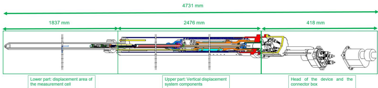
Figure 2: CARMEN device
