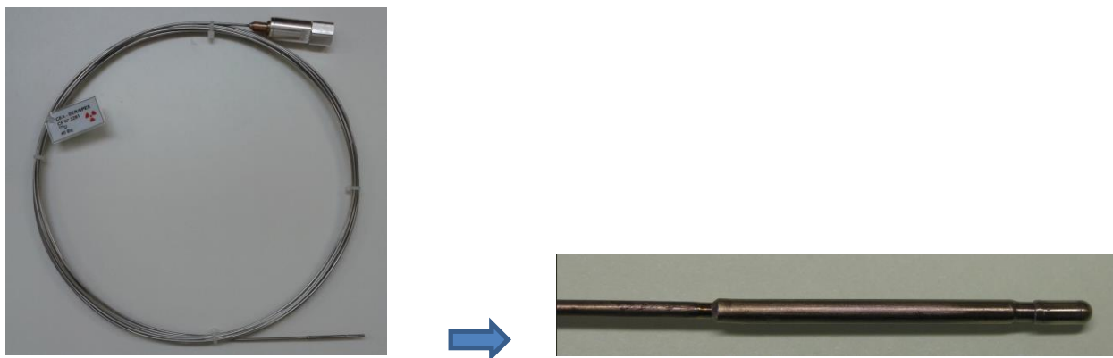
Figure 5: Miniature fission chamber
