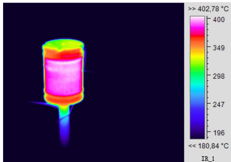
Figure 7: Thermal camera image during temperature stabilization at the landing
