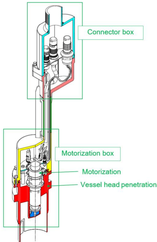
Figure 13: Mock-up of the CARMEN's head
