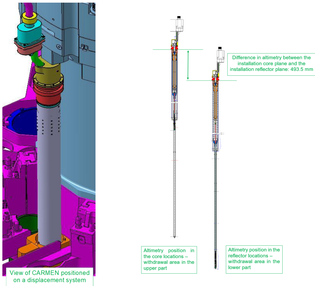
Figure 3: CARMEN design
