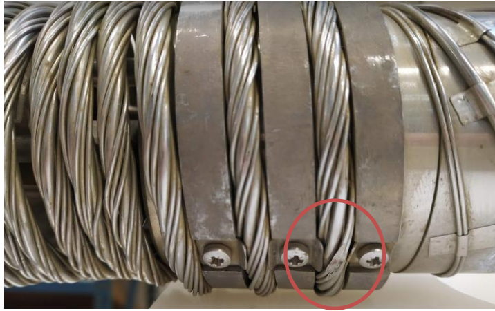
Figure 11: Indication of wear on the wiring
