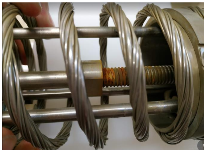
Figure 12: Traces of corrosion on the threading of the ball screw
